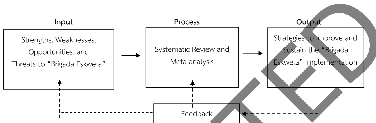
Figure 1. Conceptual Paradigm
